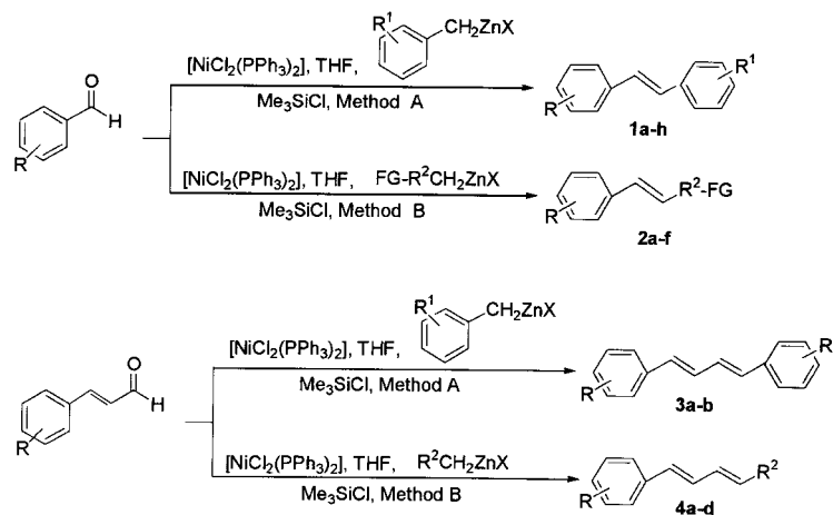
Scheme 1.
